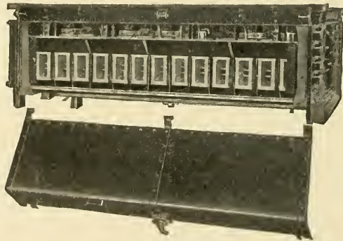
Fig. 61. Group of Sprague-General Electric Unit Switch
